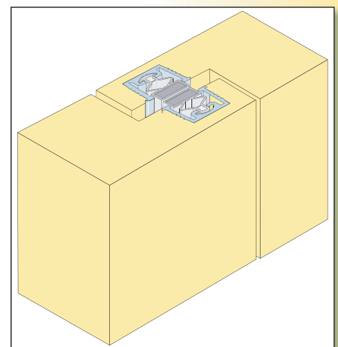
Above: Rebated meeting stile detail.
